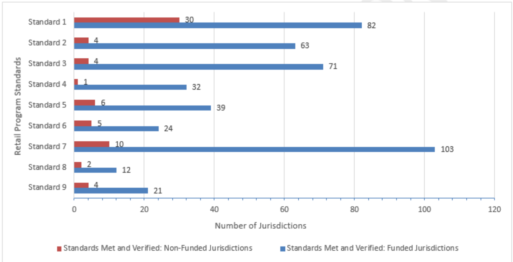
Comparison of the Number of Funded and Non-Funded Jurisdictions Enrolled in the Retail Program Standards (n=825)
